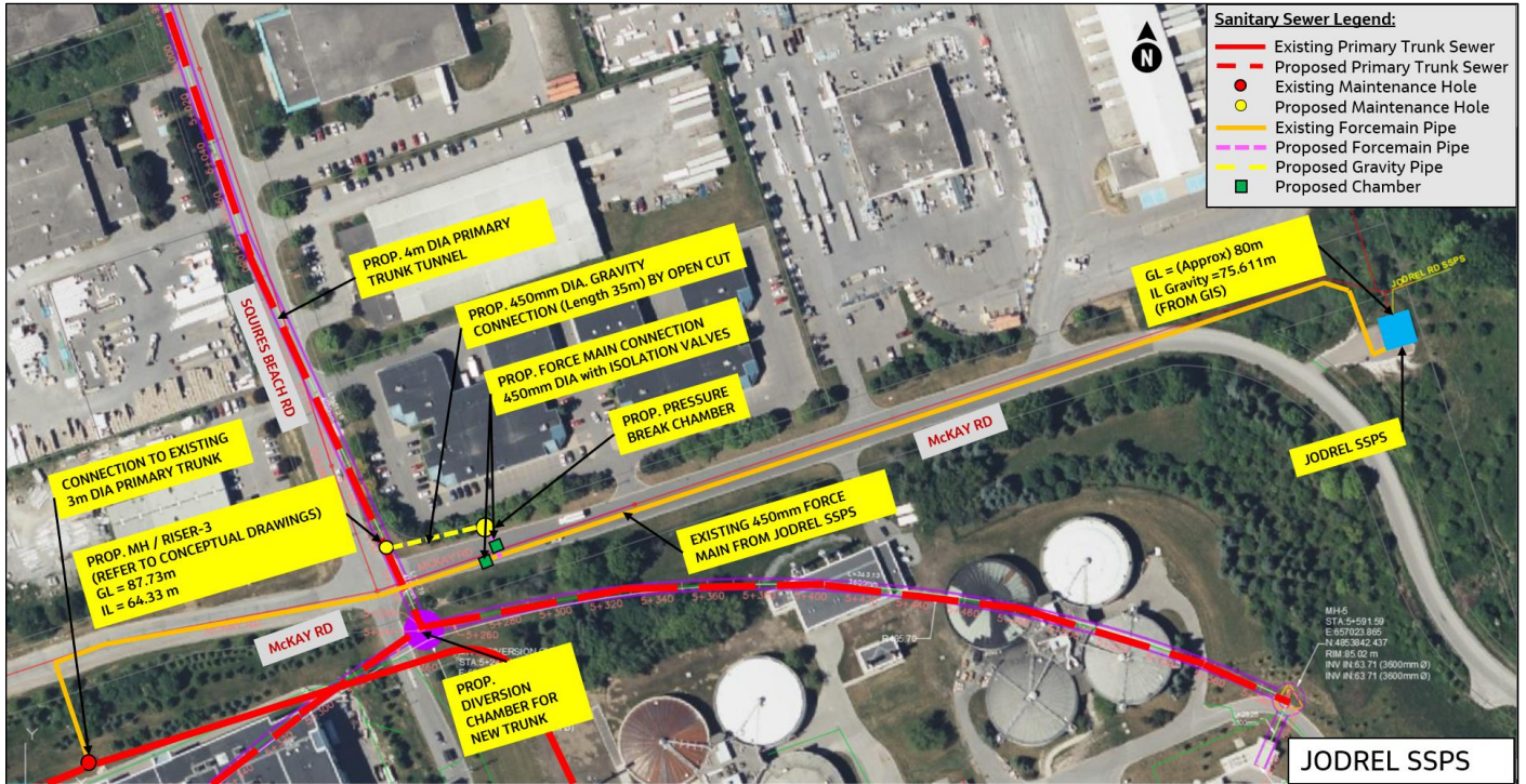
Figure 8.15 Connection of Jodrel SPS to the Proposed Primary Trunk Sewer
