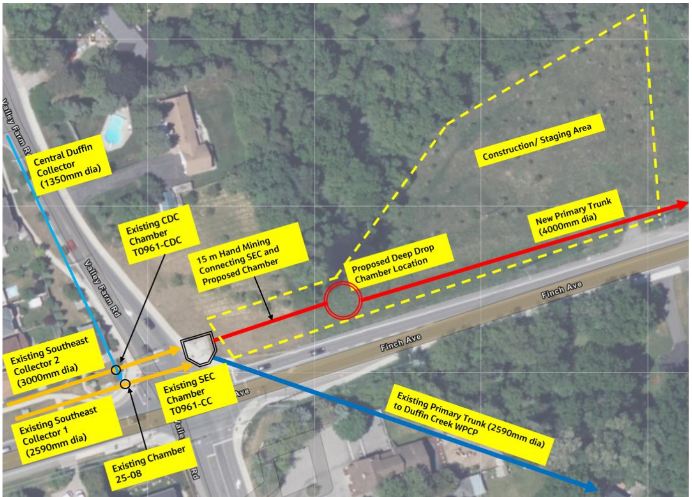
Figure 8.8 Conceptual Design Layout for the Upstream Connection of Preferred Alignment
