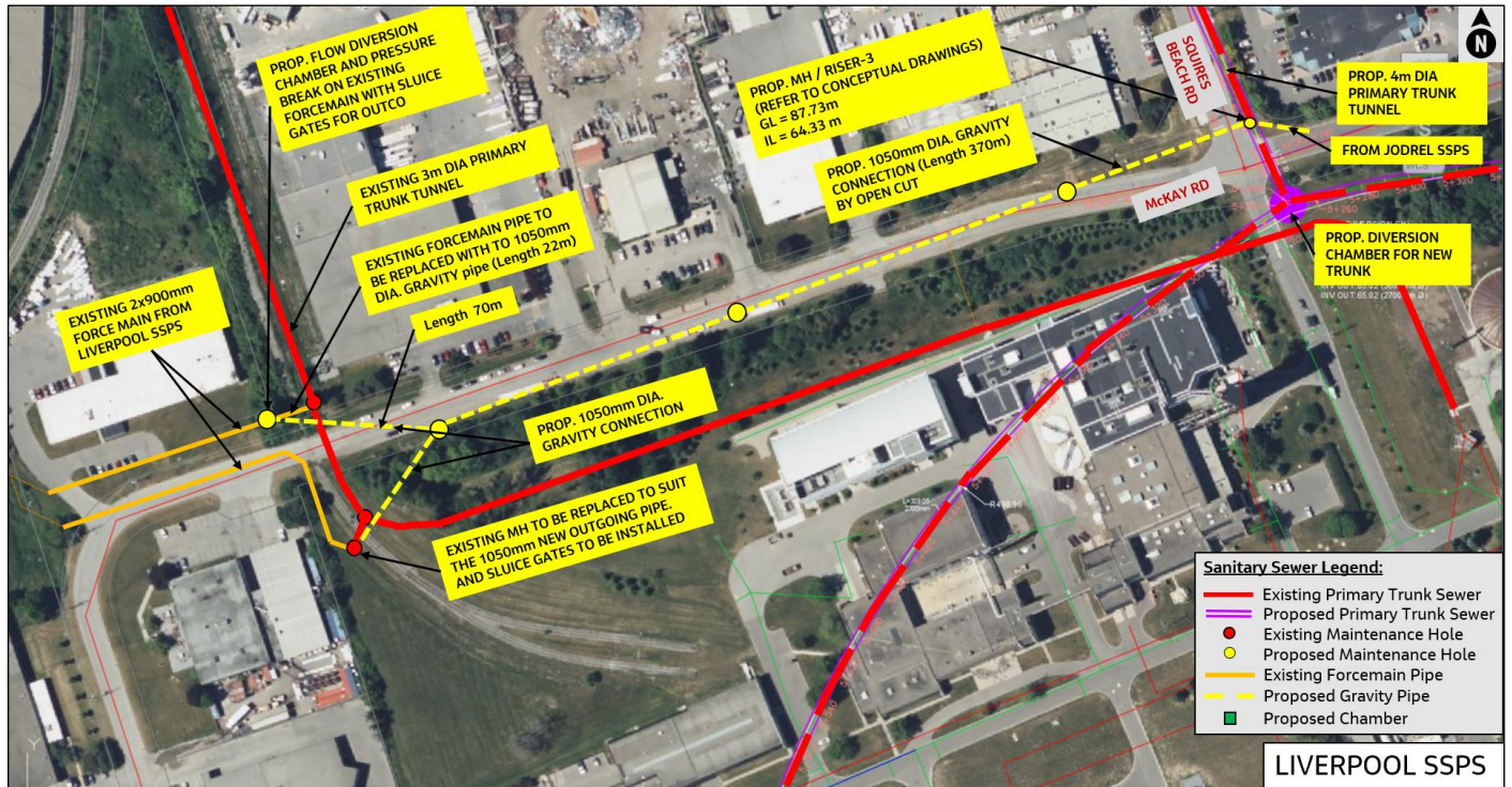
Figure 8.16 Connection of Liverpool SPS to the Proposed Primary Trunk Sewer
