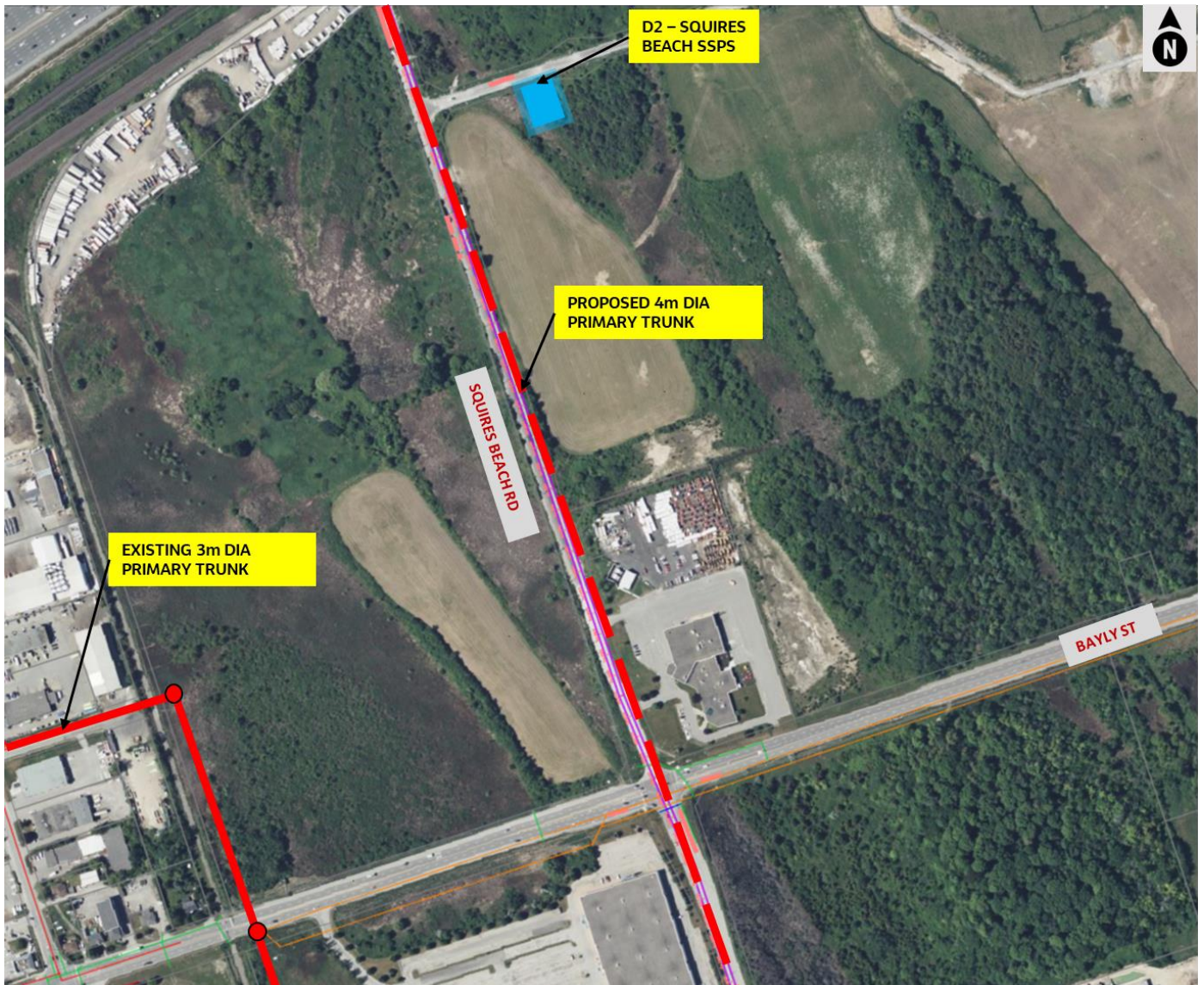
Figure 8.12 Squires Beach SPS Conceptual Schematic
