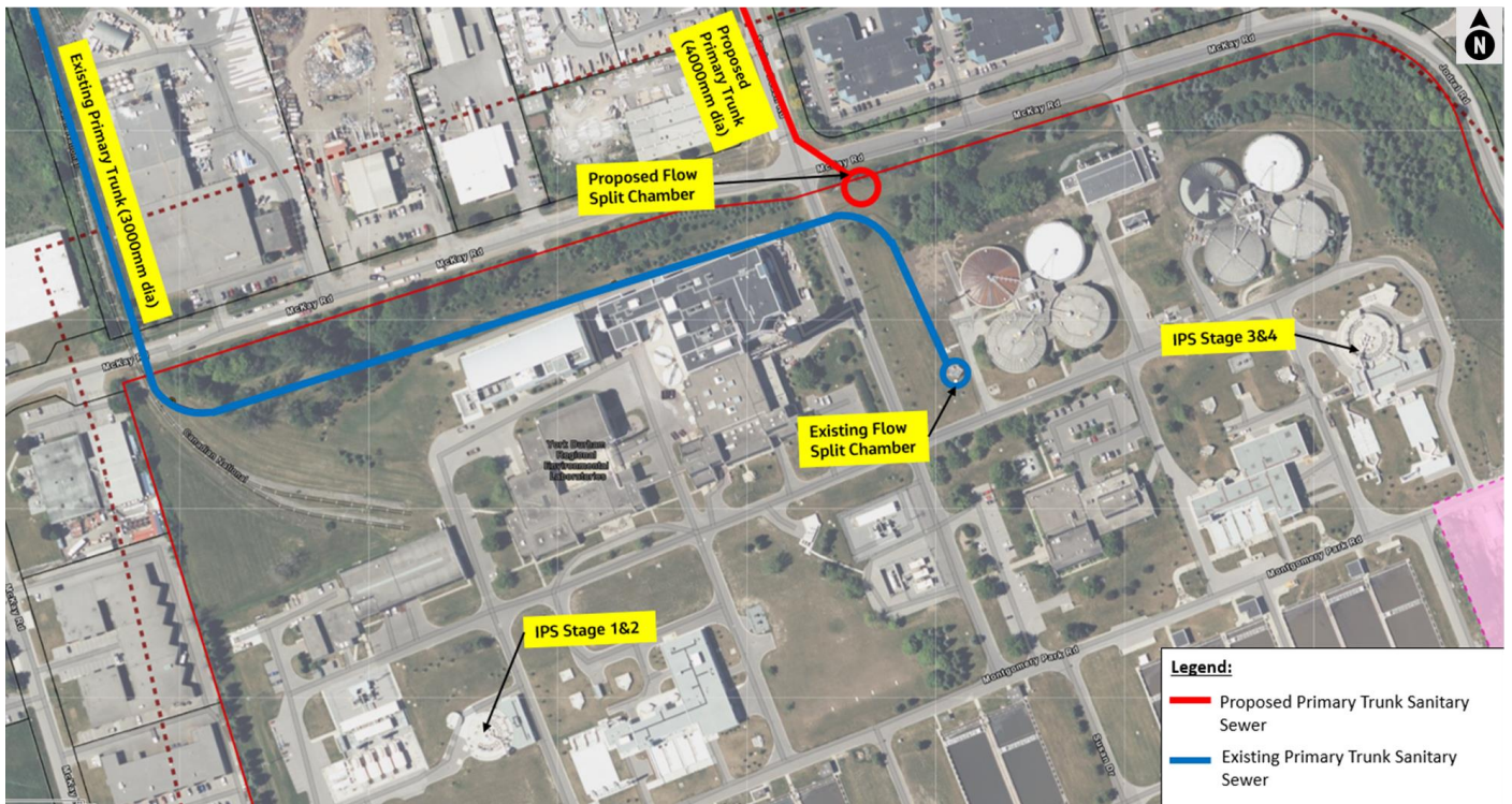
Figure 8.9 General Location and Layout of New Flow-splitting Chamber
