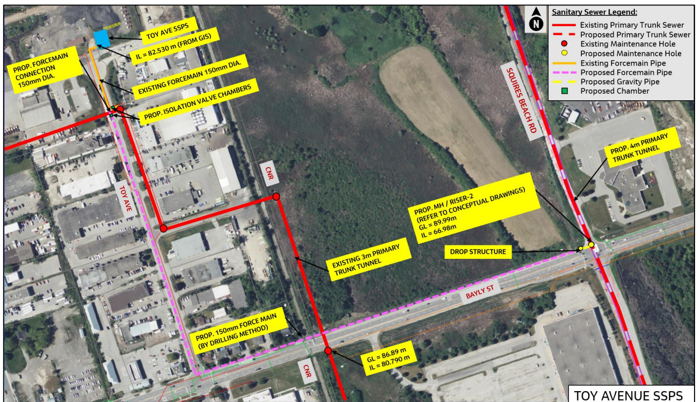
Figure 8.13 Connection of Toy Avenue SPS to the Proposed Primary Trunk Sewer
