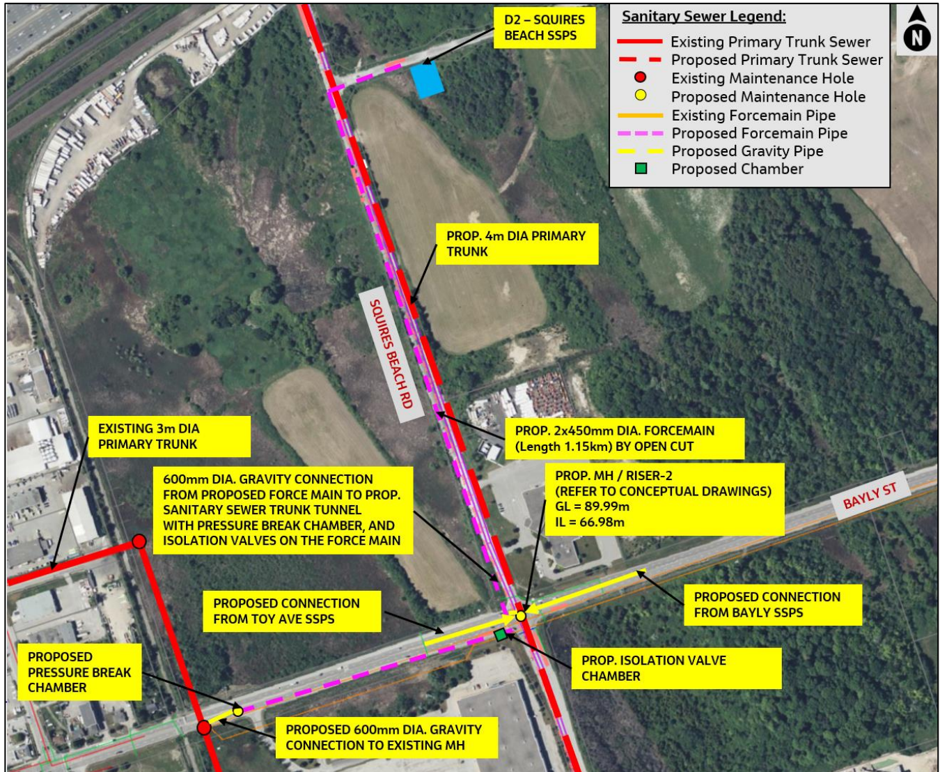
Figure 8.18 Connection of Squires Beach SPS to the Existing and Proposed Primary Trunks
