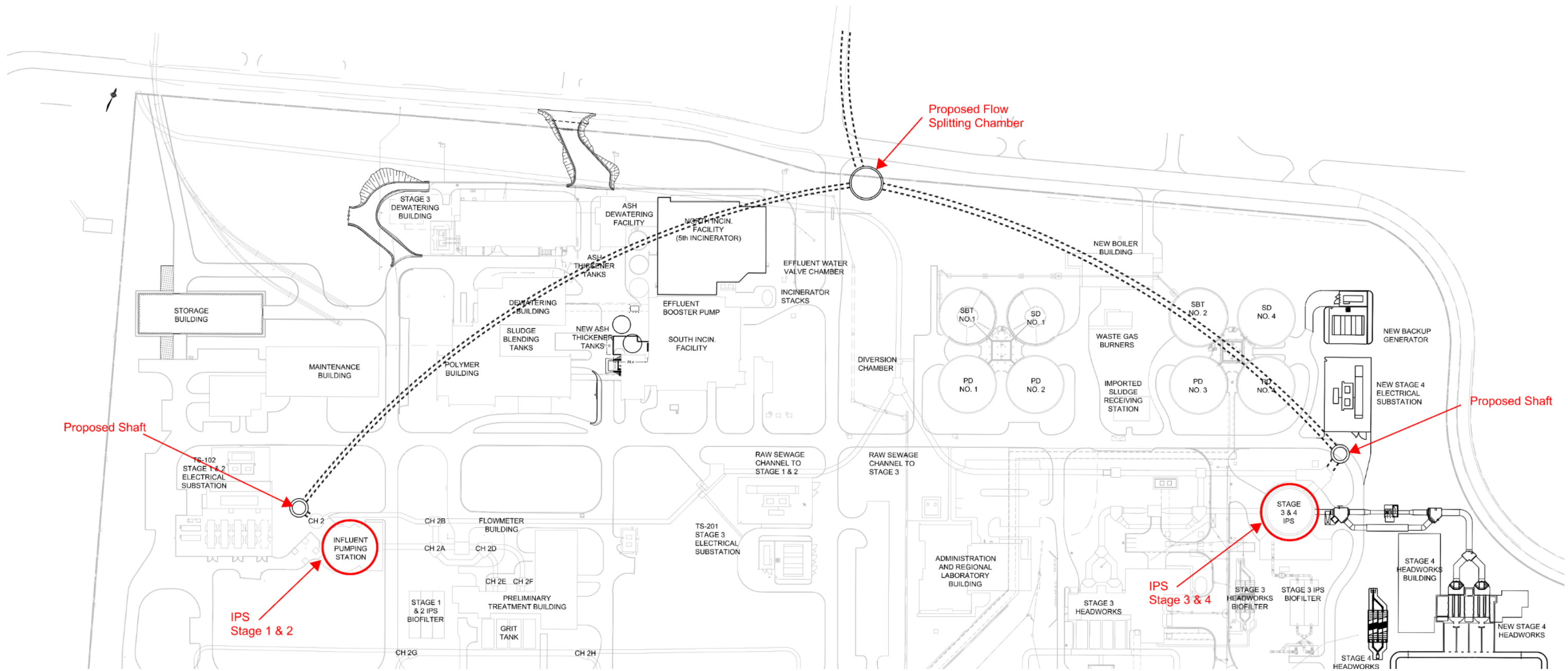
Figure 8.10 Primary Trunk Connections at the Duffin Creek WPCP Influent Pumping Stations
