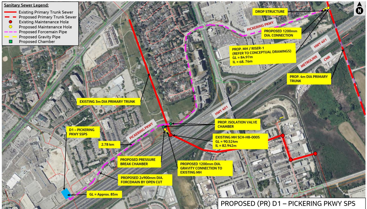
Figure 8.17 Connection of Pickering Parkway SPS to the Existing and Proposed Primary Trunks
