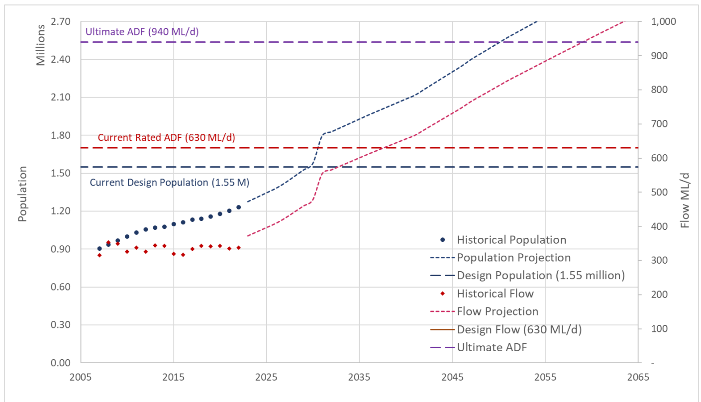
Figure 9.12 Population and Flow Projections for Duffin Creek WPCP
