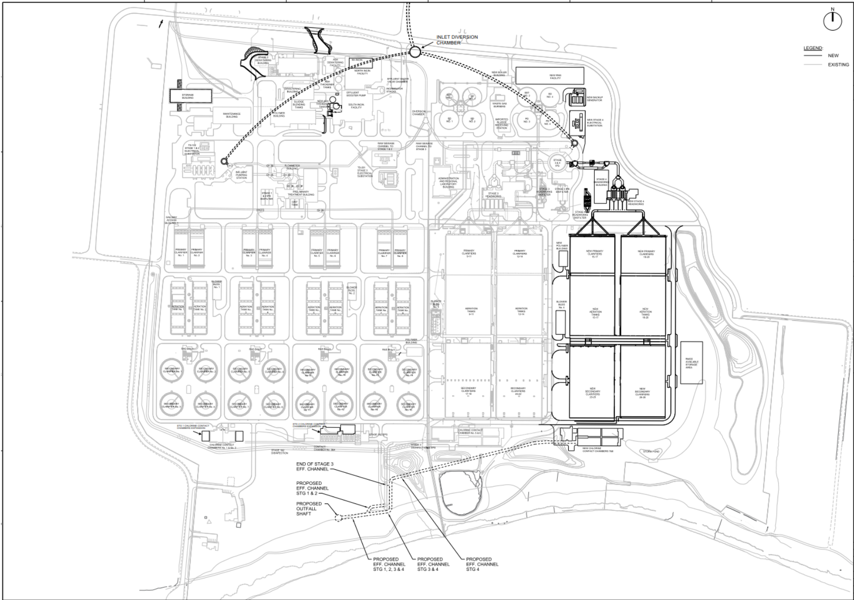
Figure 9.13 Duffin Creek WPCP Site Layout for the Plant Capacity Expansion
