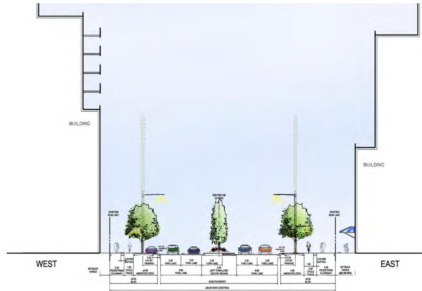
Figure 107: Concept C | Section B-B Steeles Gateway Mid-block
