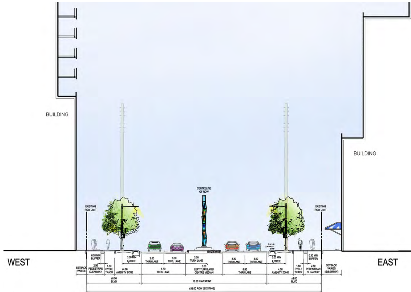
Figure 105: Concept C | Section A-A Steeles Gateway Median
