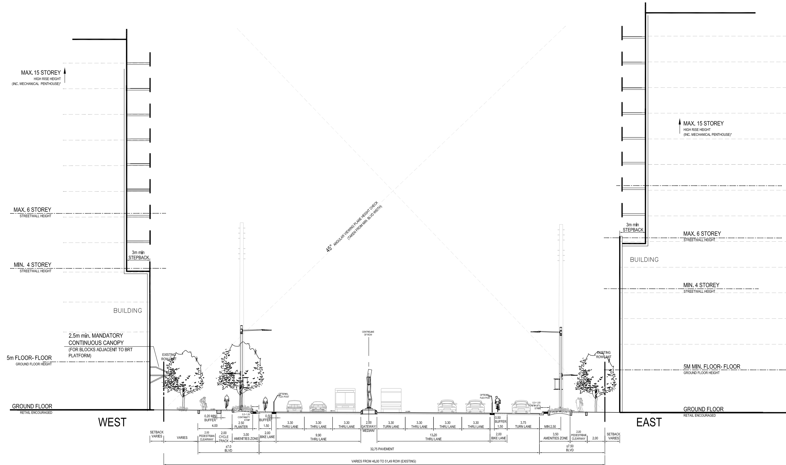
Figure 91: Urban Criteria - Richmond Hill Centre District
