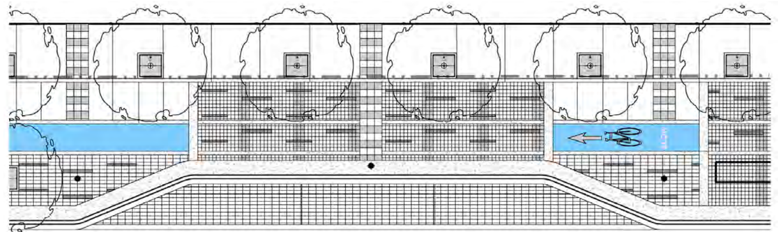
Figure 48: Typical Lay-By Parking Bay in-line with Furnishing and Planting Zone
