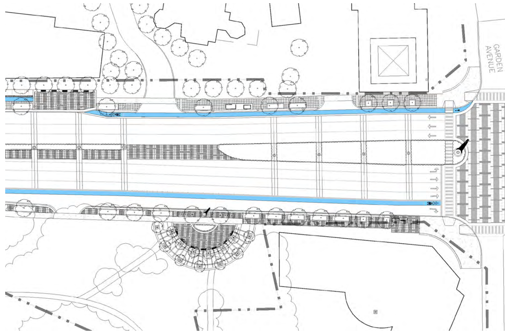
Figure 178: Detail Area Plan - Richmond Hill Centre
