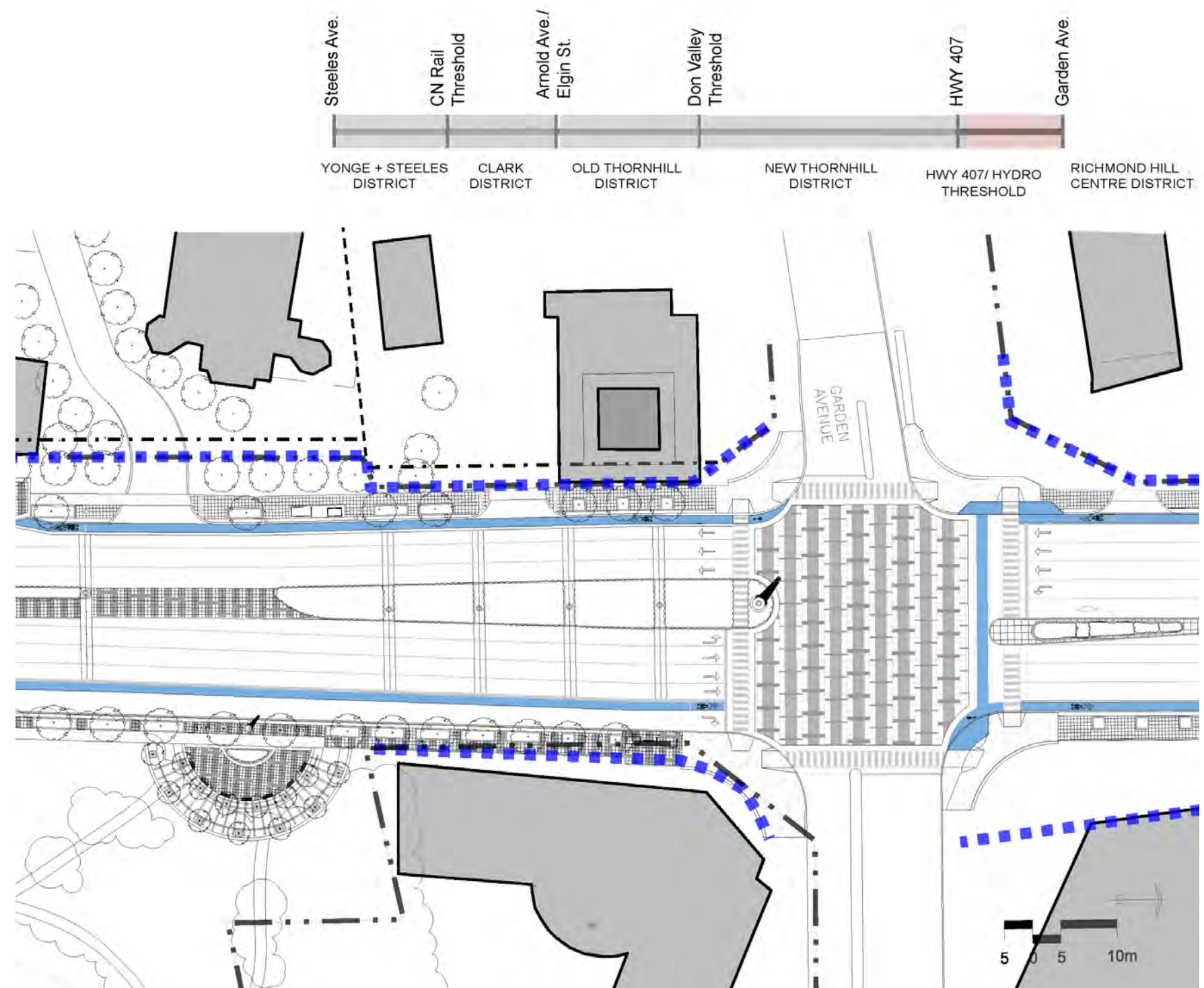
Figure 90: Typical Detail Plan of Richmond Hill Centre District
