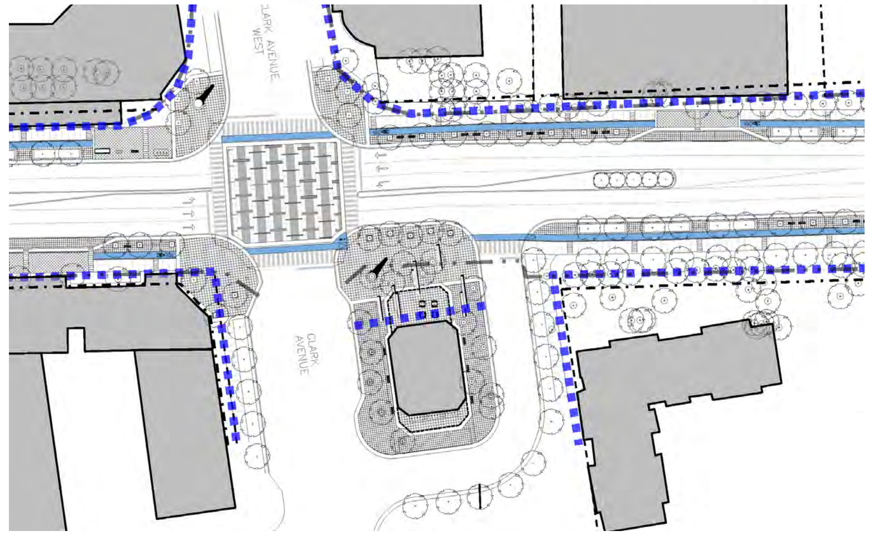
Figure 64: Typical Detail Plan of Clark Station District
