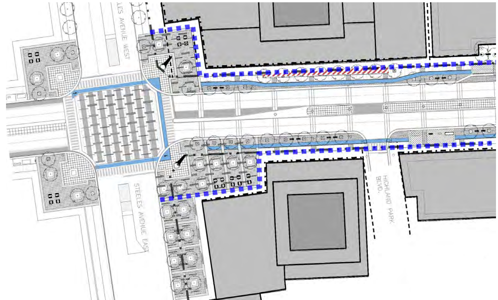
Figure 60: Typical Detail Plan of Yonge Steeles Gateway District
