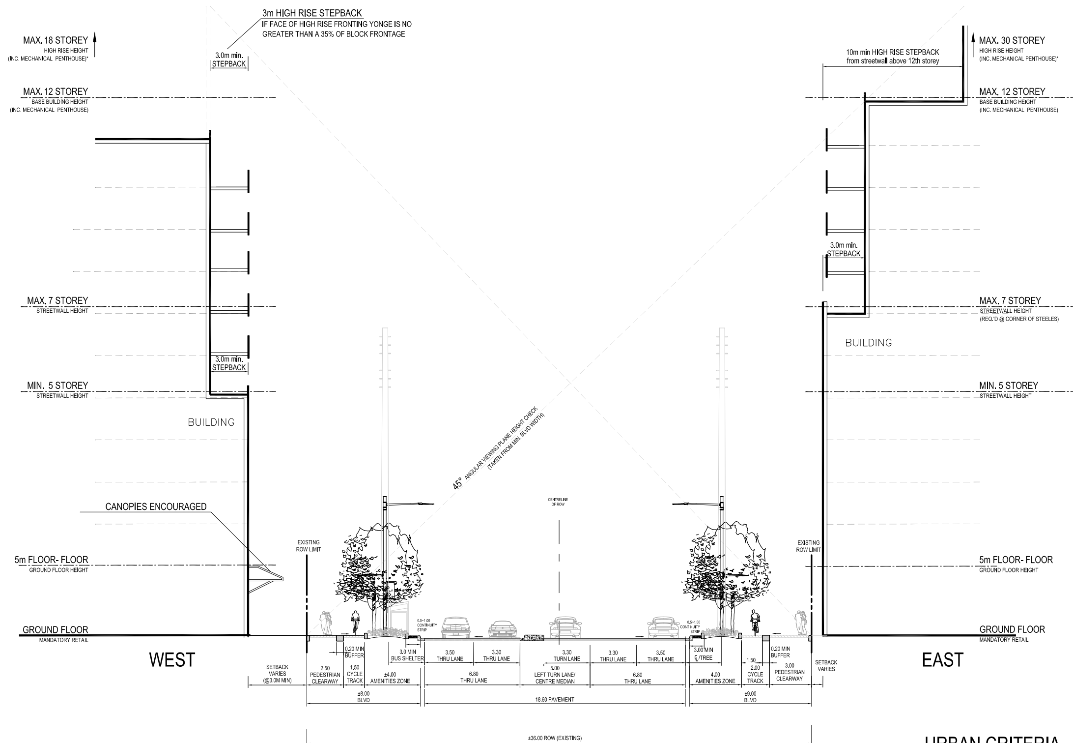
Figure 65: Urban Criteria - Clark District: Mid-block
