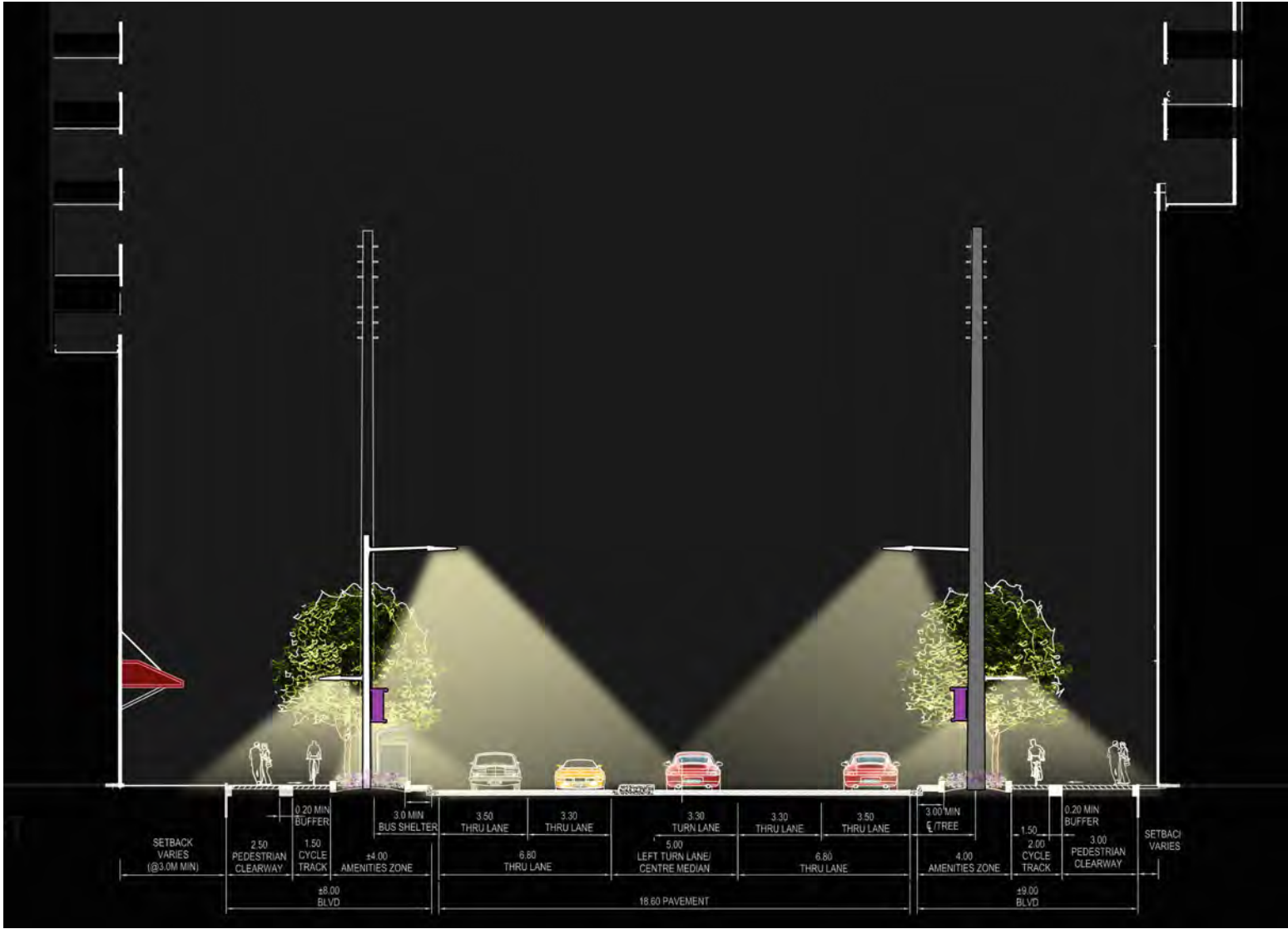
Figure 18: Typical Lighting Cross-Section
