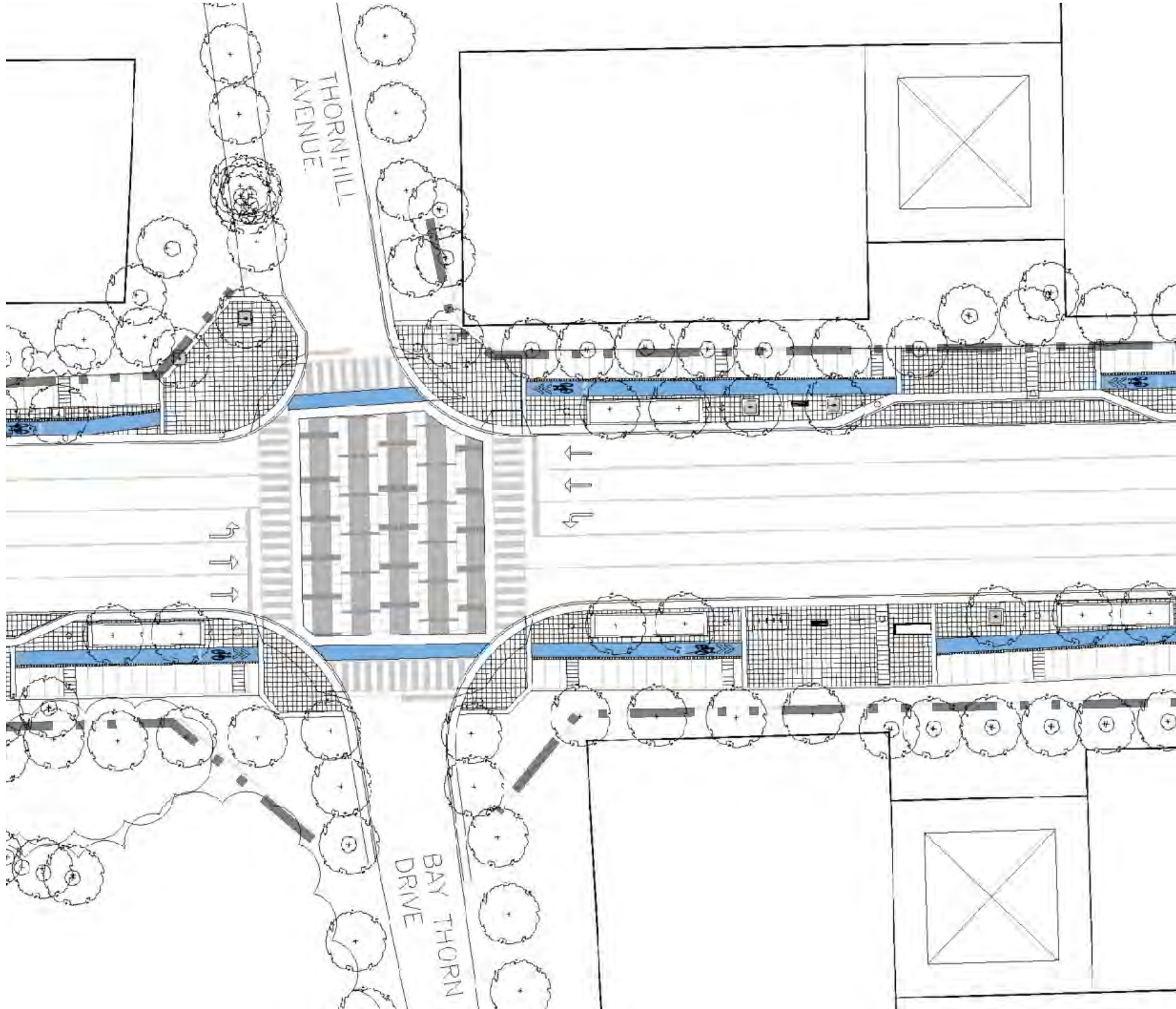
Figure 160: Intersection Detail Area Plan - New Thornhill District
