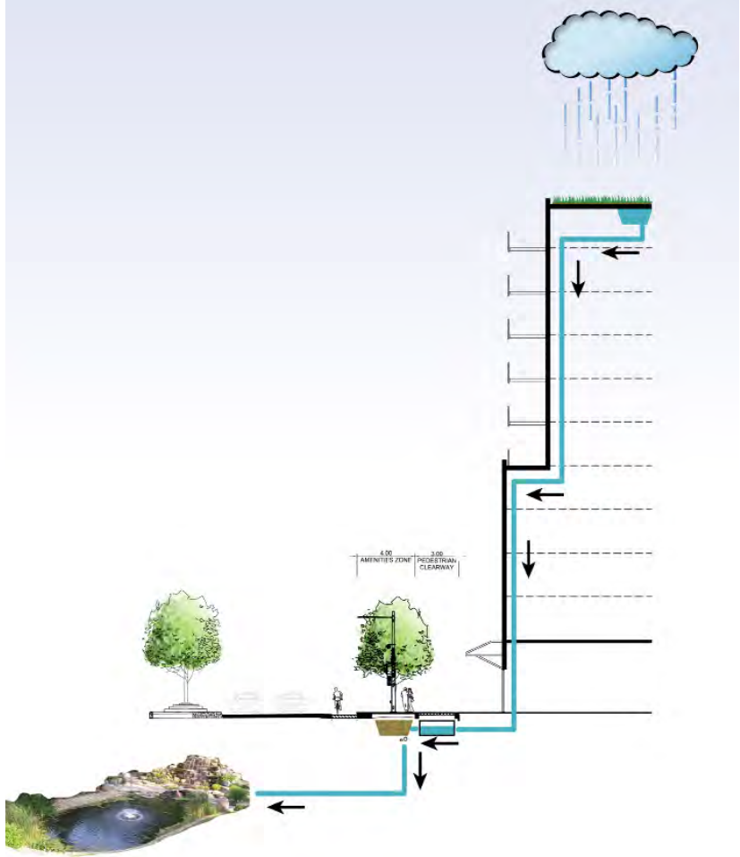
Figure 27: Stormwater Management and Drainage System Diagram
