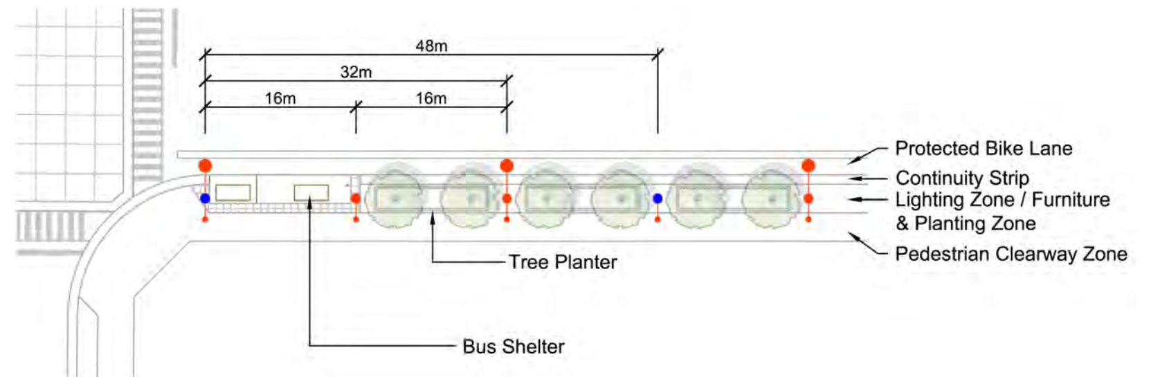
Figure 20: Lighting Concept 2 (Hydro Located Overhead)
