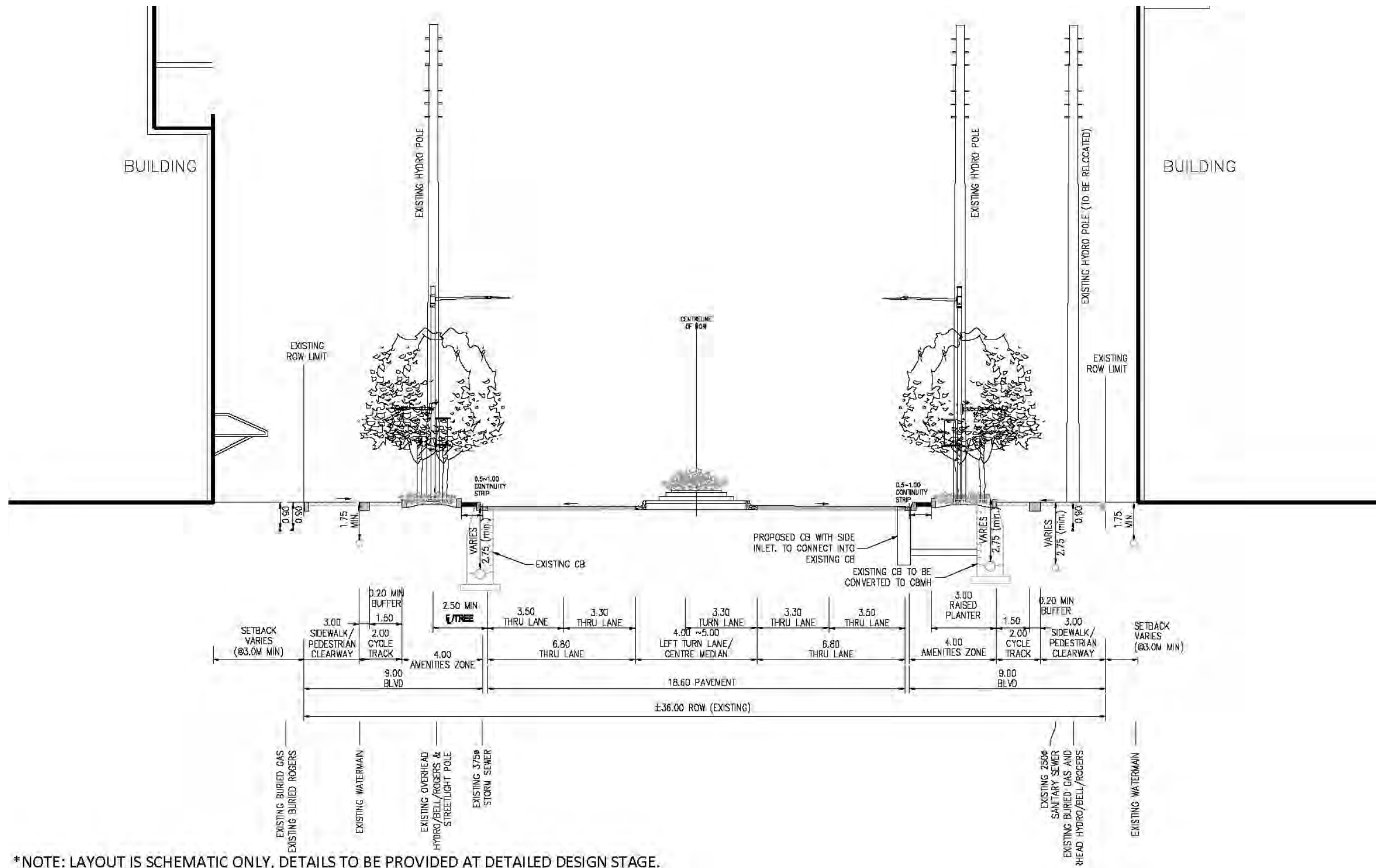
Figure 218: Section D-D Clark District
