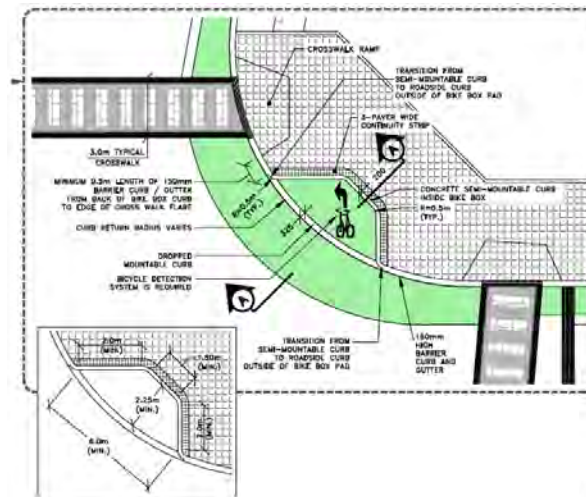
Figure 29: Typical Bike Box D-10.04. Source: York Region Pedestrian & Cycling Planning & Design Guidelines
