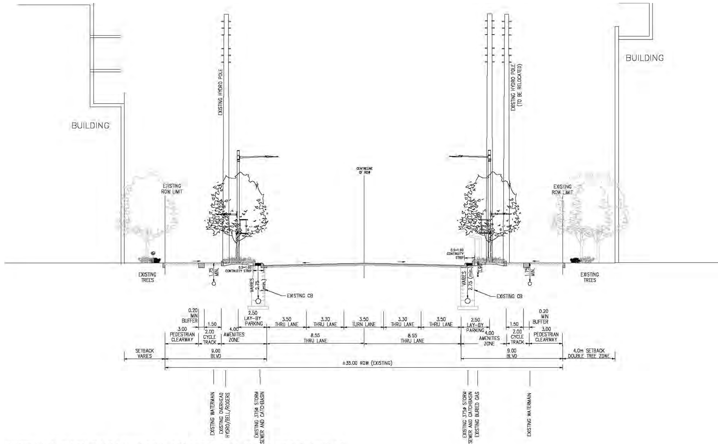
Figure 222: Section H-H New Thornhill
