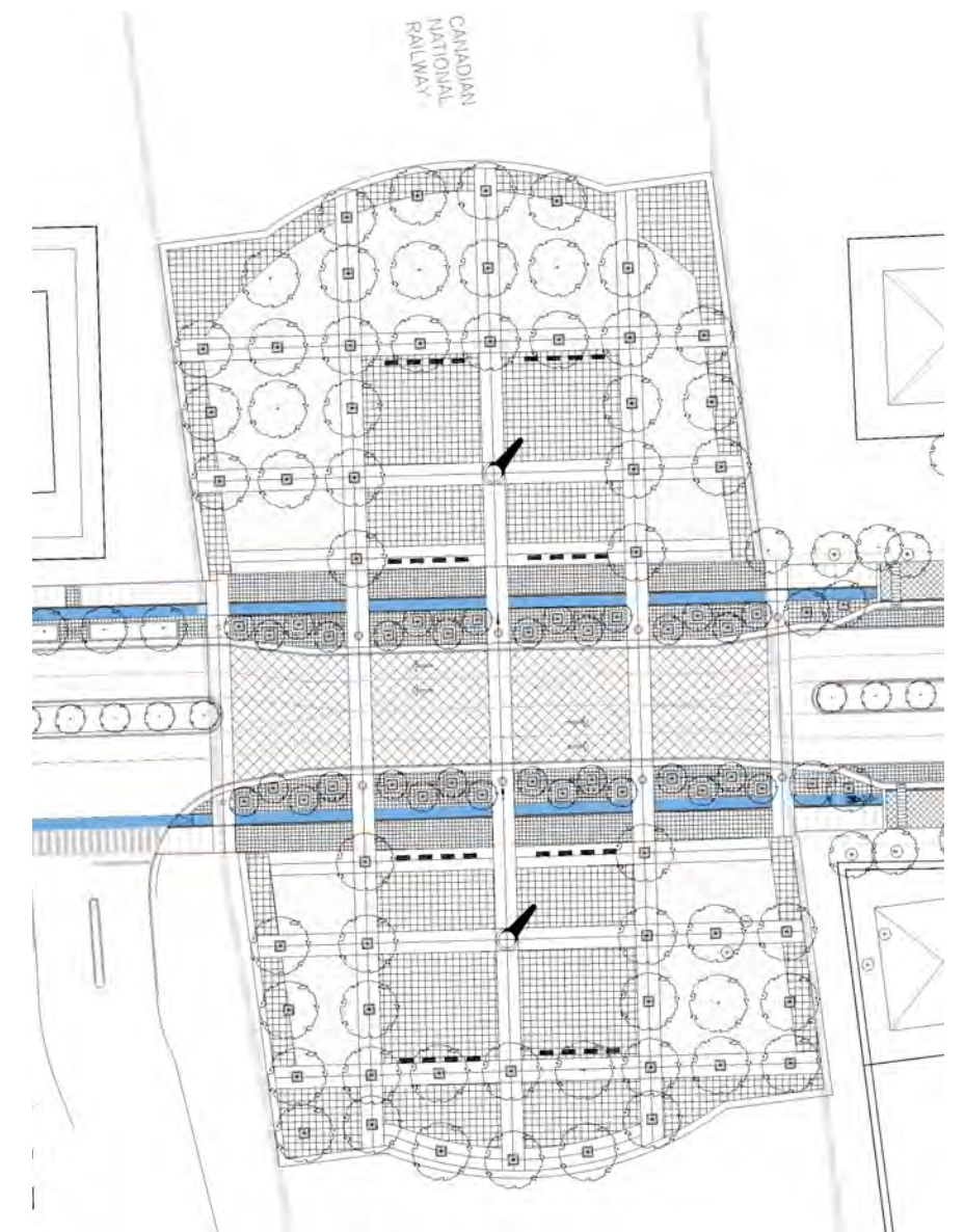
Figure 108: Detail Plan - CN Rail Bridge
