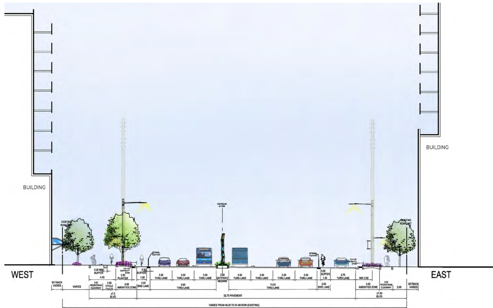
Figure 182: Concept C | Section J-J Richmond Hill Centre District: Transition to Existing Conditions at Garden Avenue
