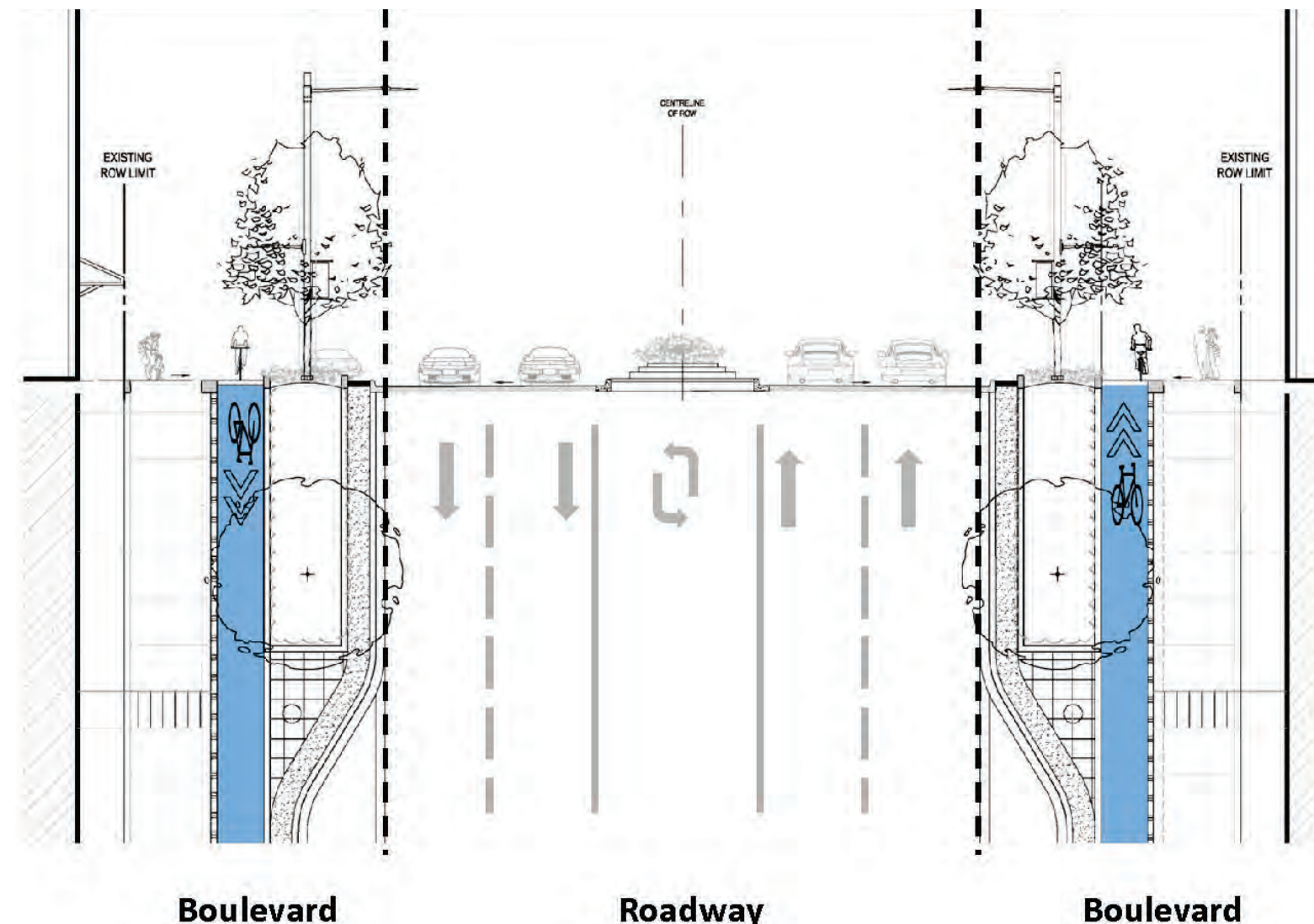
Figure 10: Typical Right-Of-Way Zones
