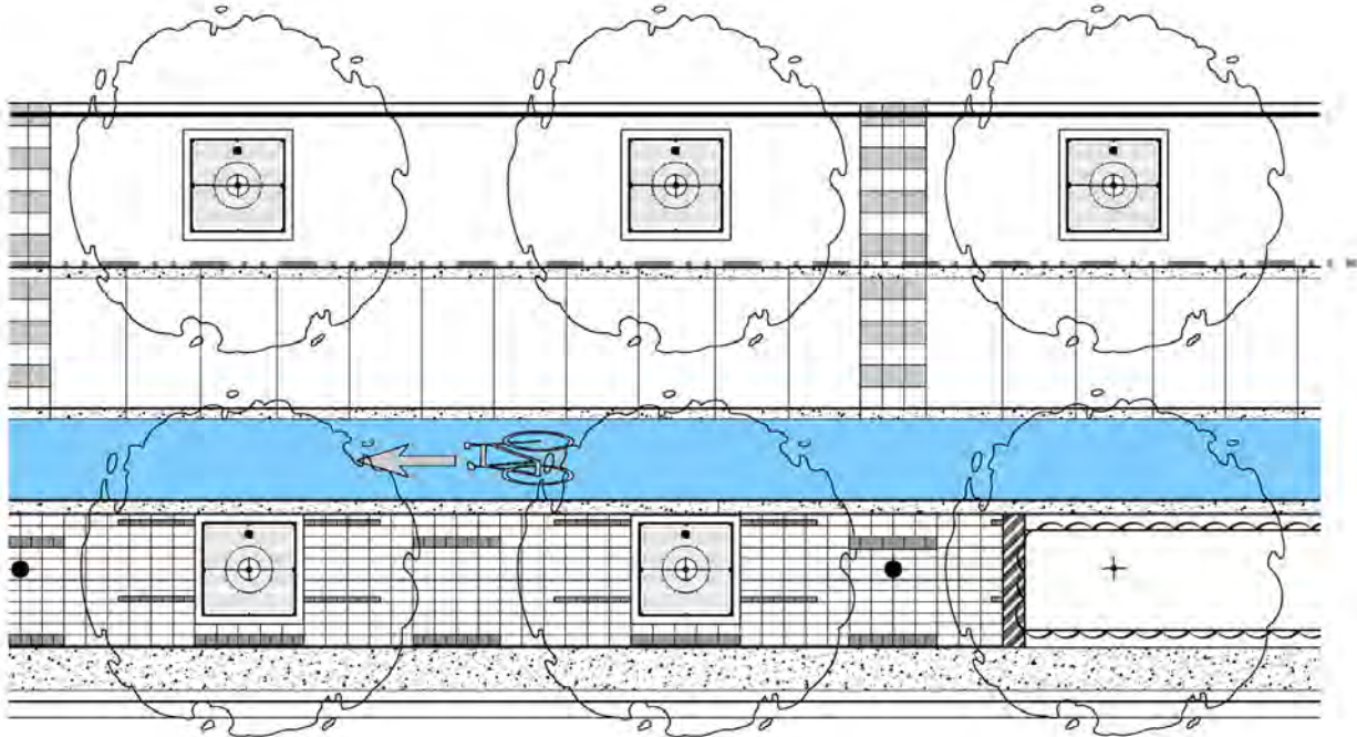
Figure 41: Pedestrian Clearway Zone Location in Boulevard
