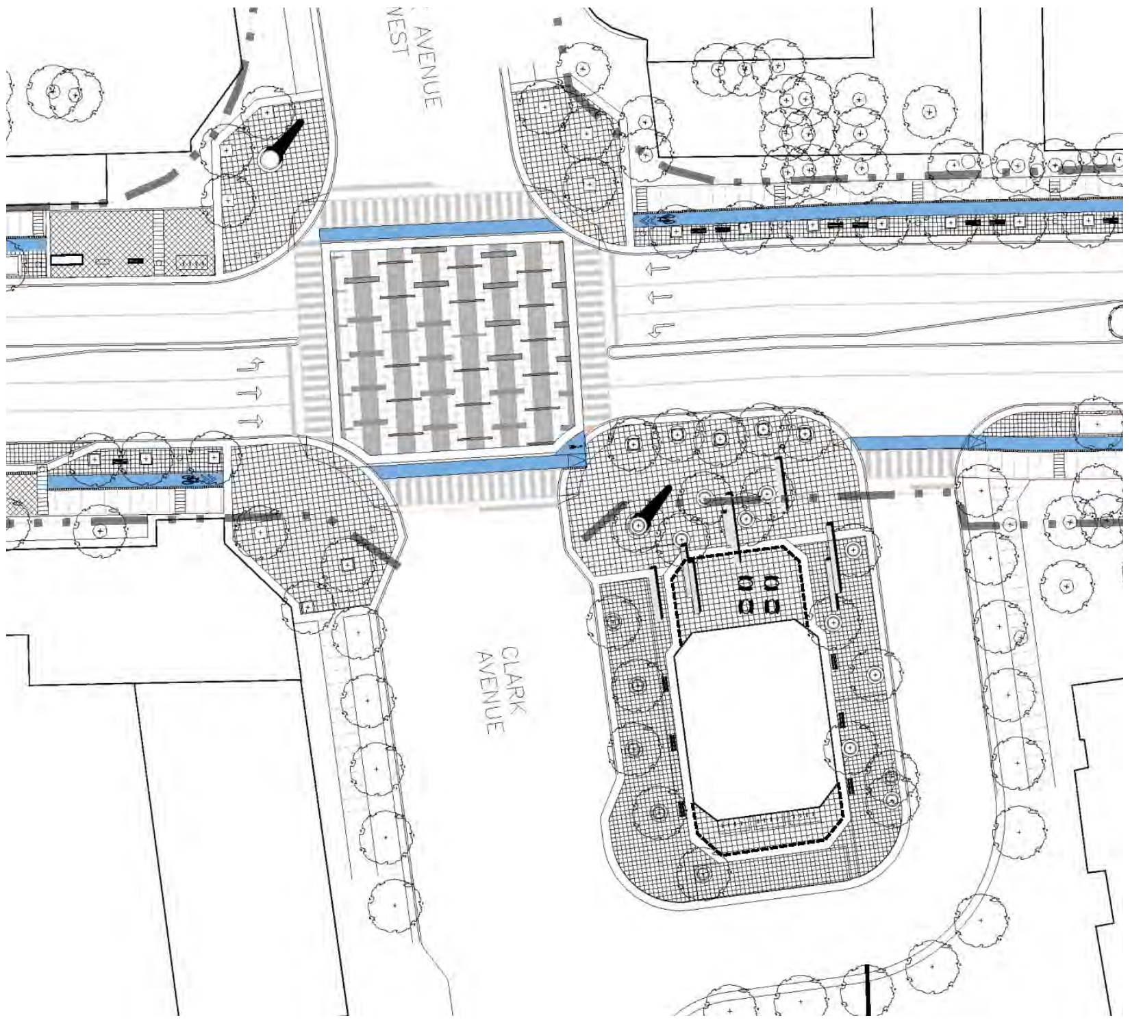
Figure 124: Intersection Detail Area Plan - Clark Station
