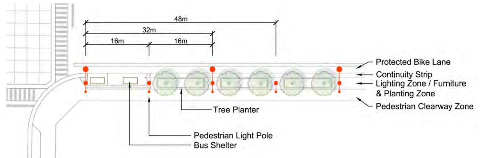
Figure 19: Lighting Concept 1 (Hydro Located Below Grade)
