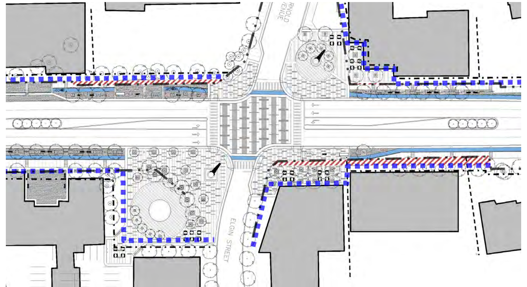
Figure 69: Typical Detail Plan of Old Thornhill District
