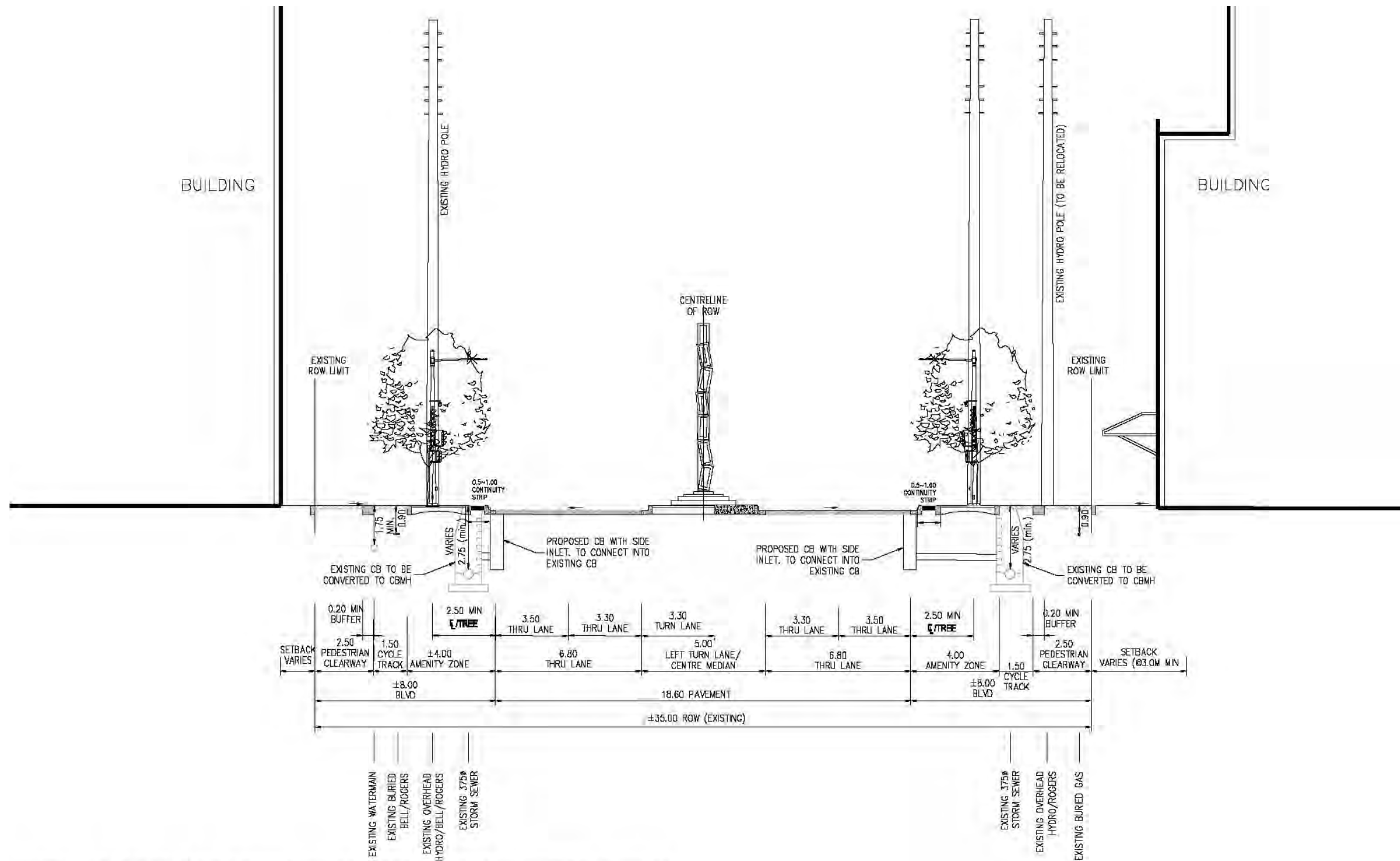
Figure 215: Section A-A Steeles Gateway Median
