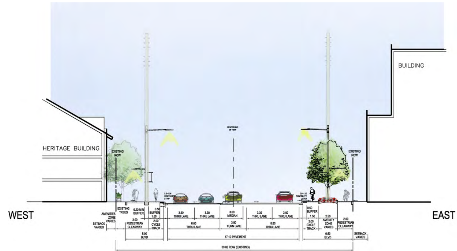
Figure 144: Concept C | Section F-F Old Thornhill (Heritage)
