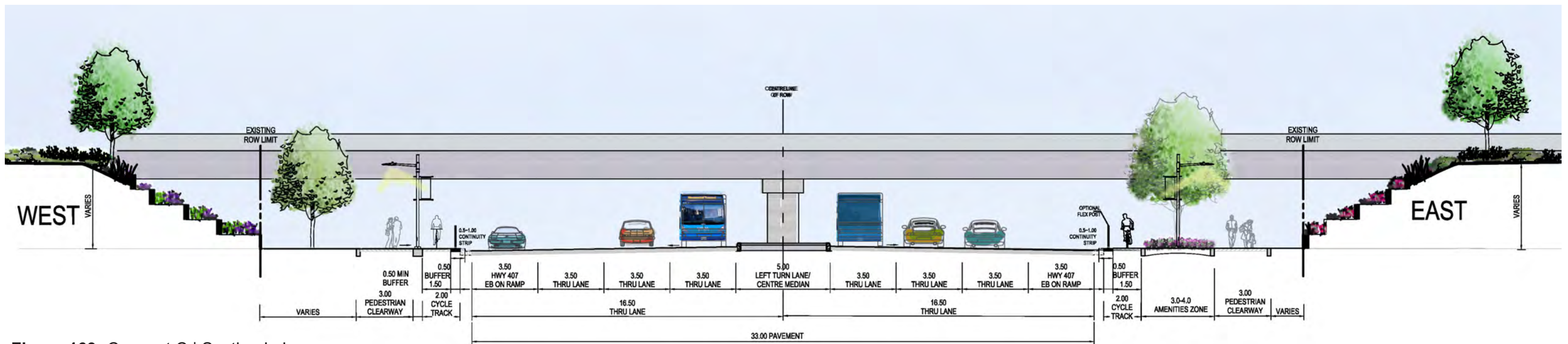
Figure 169: Concept C | Section I2-I2 Approaching 407 @ Langstaff Road East
