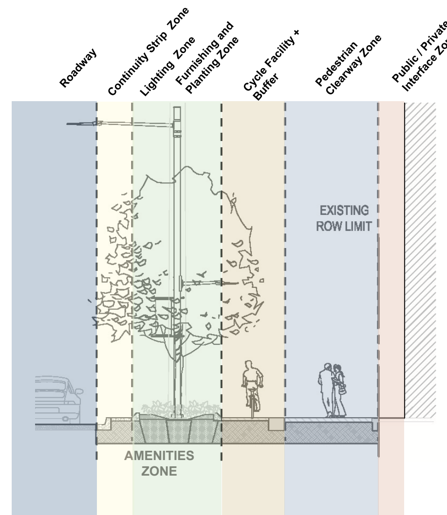
Figure 14: Typical Cross-Section of Boulevard
