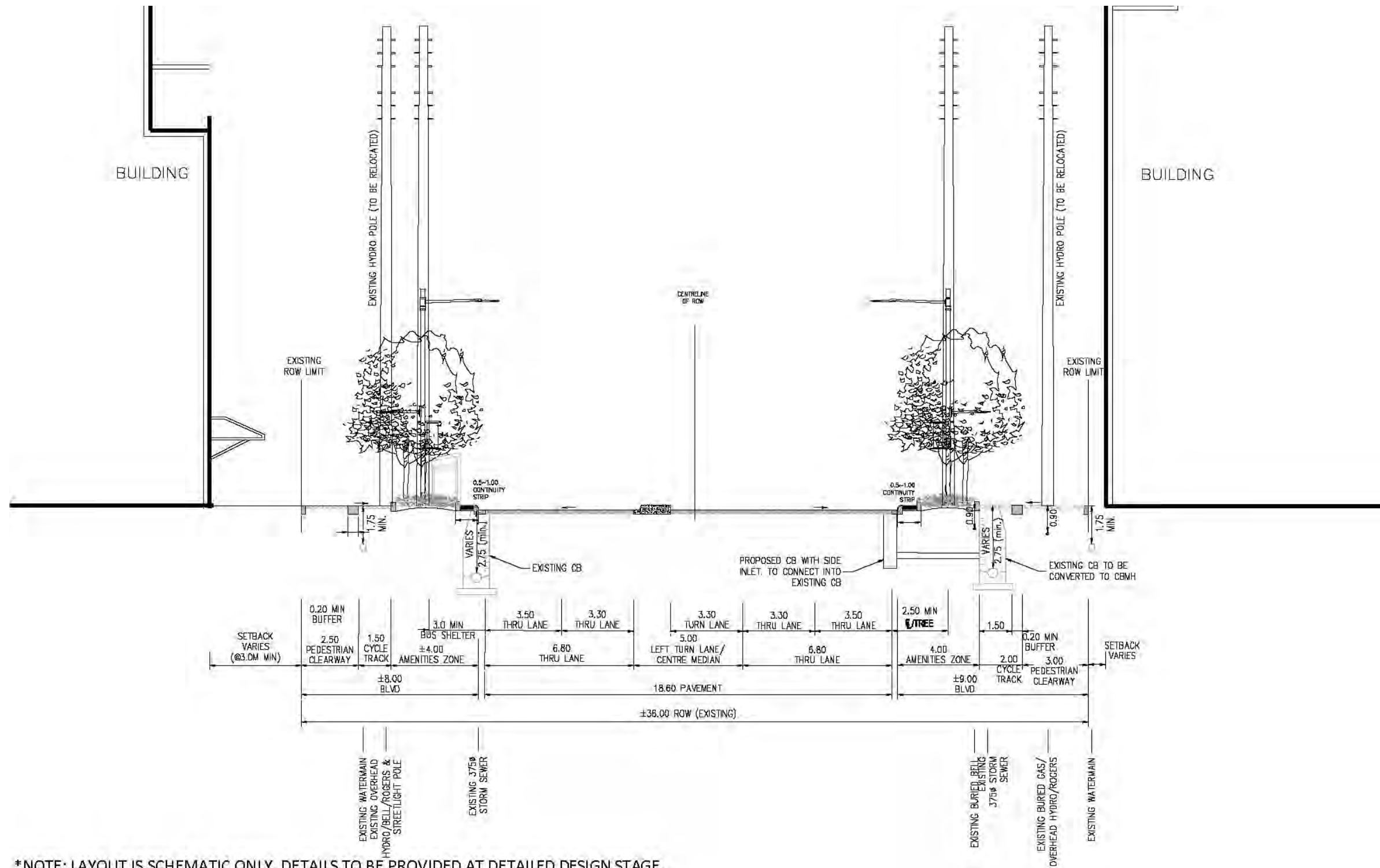
Figure 217: Section C-C Clark District Mid-block
