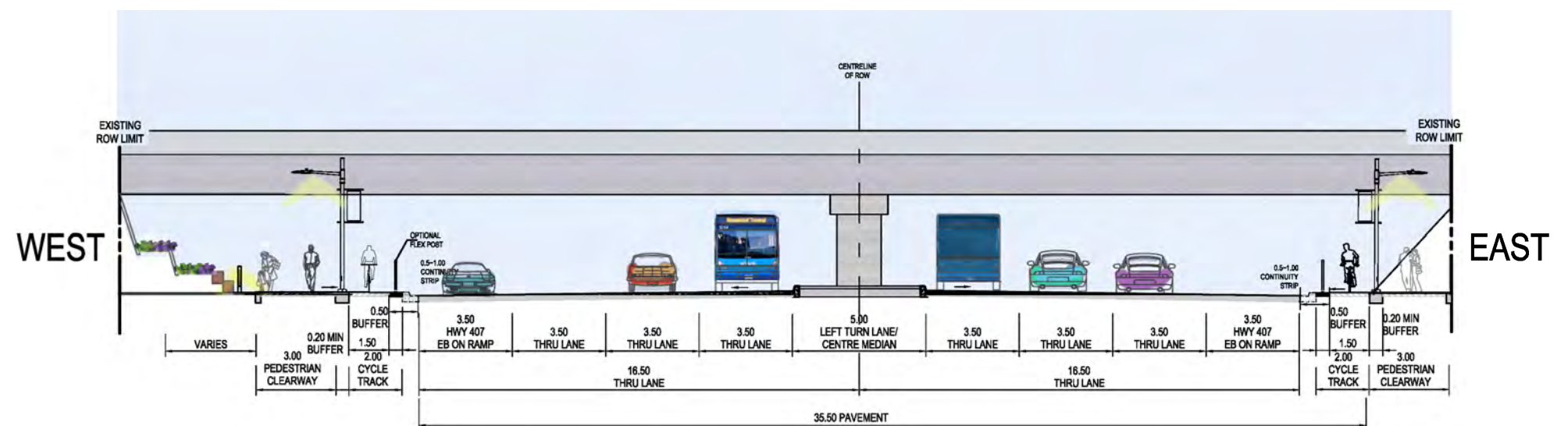
Figure 164: Concept C | Section I1-I1 407 w/Reduced Shoulder
