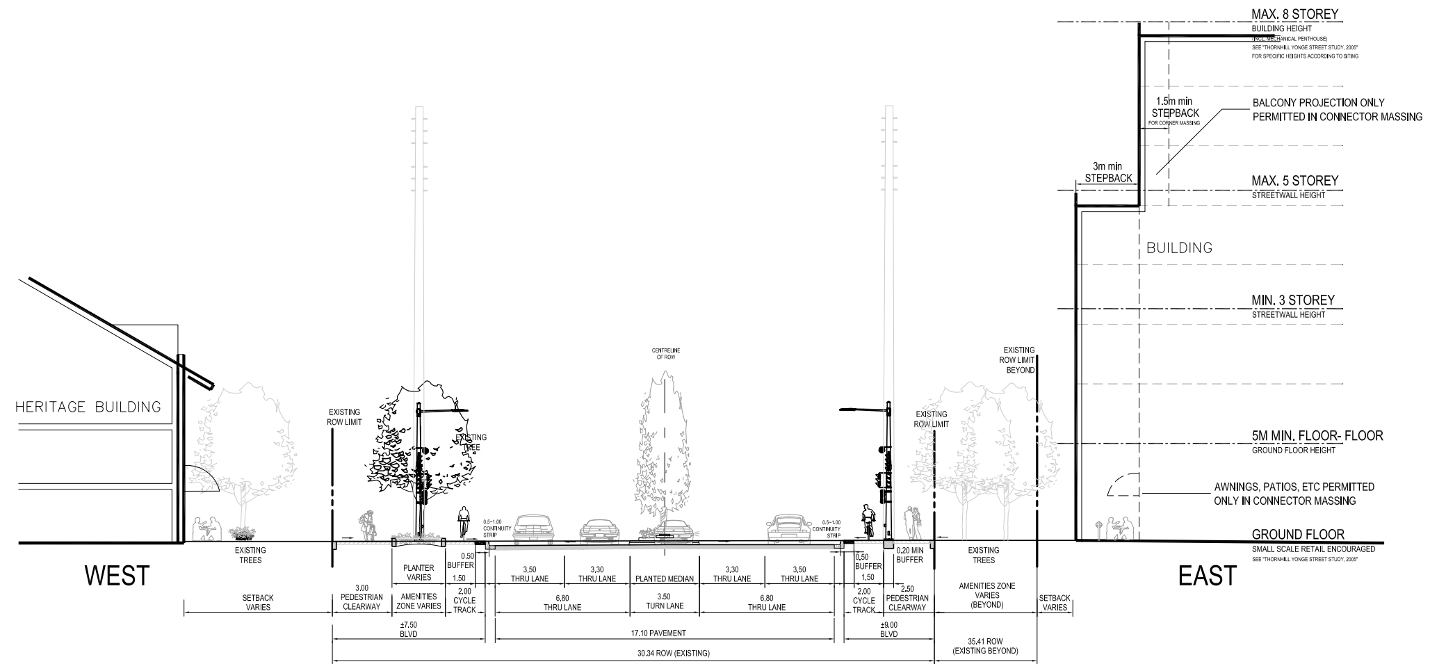
Figure 70: Urban Criteria - Old Thornhill: Approach to Intersection
