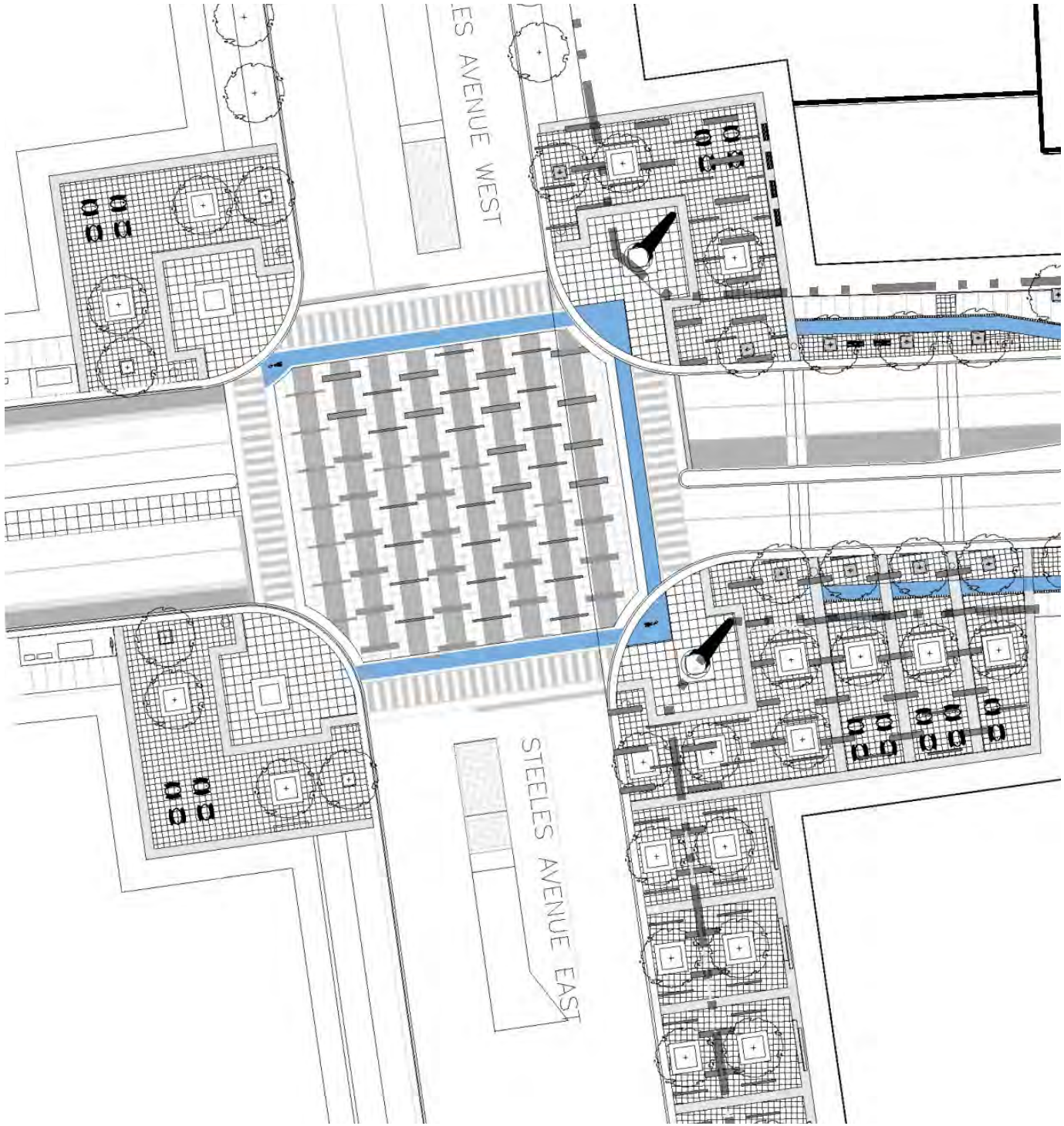
Figure 102: Intersection Detail Area Plan - Yonge Steeles Gateway
