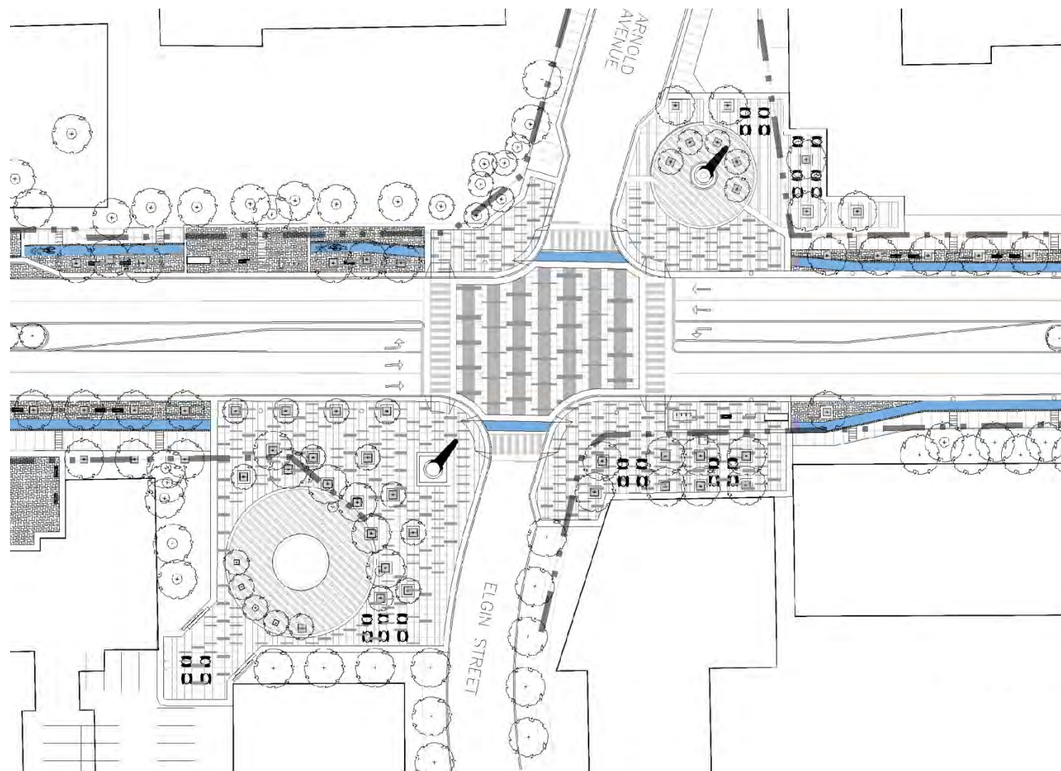
Figure 138: Intersection Detail Area Plan - Old Thornhill District
